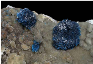
Veselyite - Sanguozhuang, CHINA Main rosette: 1.1 x 1 cm
