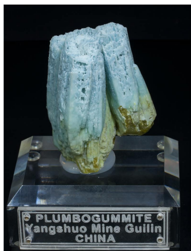
Plumbogummite - Yangshuo, CHINA 5.6 x 4 x 2.7 cm
